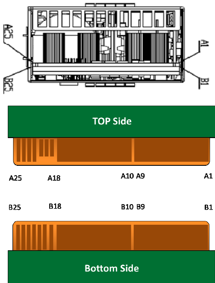
Figure 4 – Card Edge Pin Out Location
