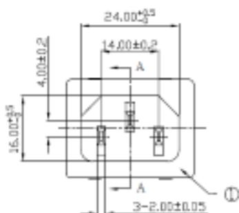
Figure 1: AC Inlet
