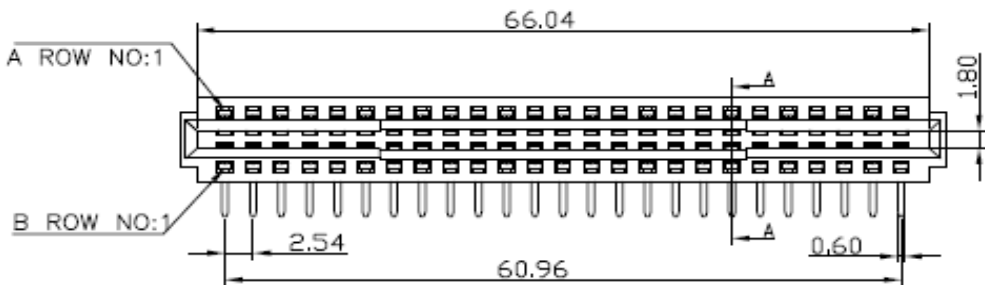
Figure 3: DC Connector
